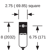
Model RCF-8 Panel Cutout Pattern
