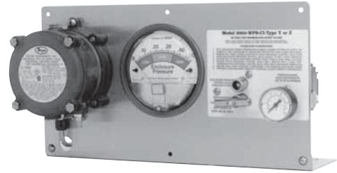
Model 3004-WPS-CI-YZ-HMT Horizontal Mount Configuration
