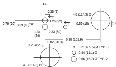
Model 3004 CK System Panel Cutout Pattern
